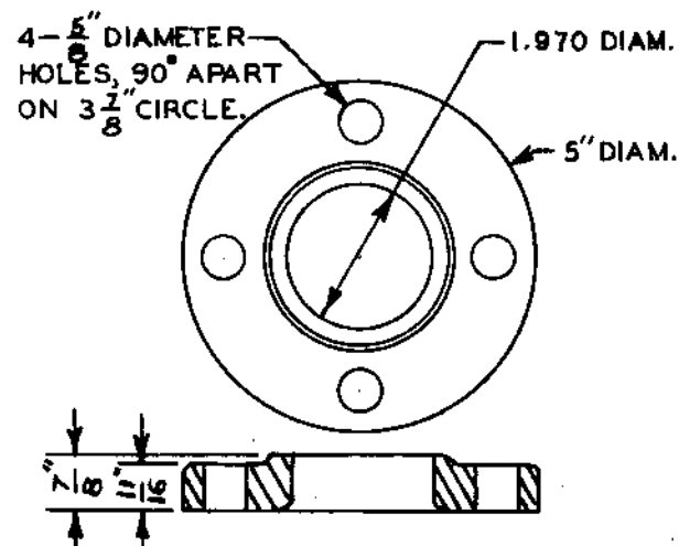
Flange(Special), Part 175-11(Modification 3). Use with Body (Special), Part 175-10(Modification 3). This flange is a 1 1/2" 150 pound American Standard lap joint flange.
