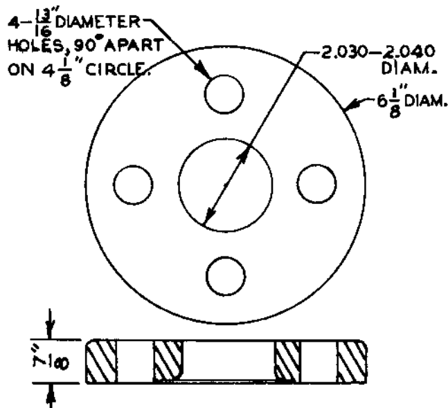
Flange(Special), Part 175-11(Modification 1). Use with Body (Special), Part 175-10(Modification 1).
