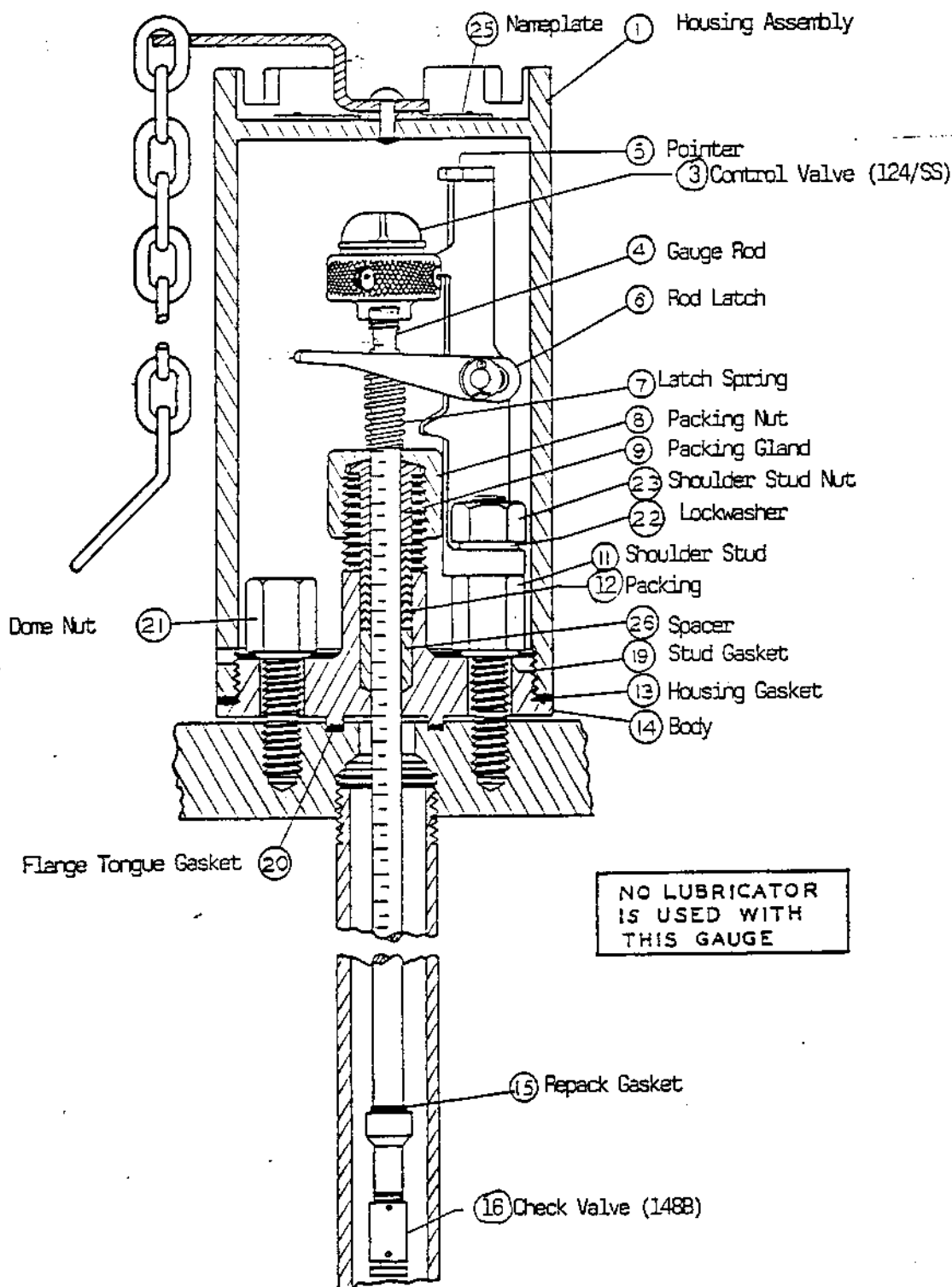
MGM TANK GAUGE NO. 62B (MODIFICATION W4)
